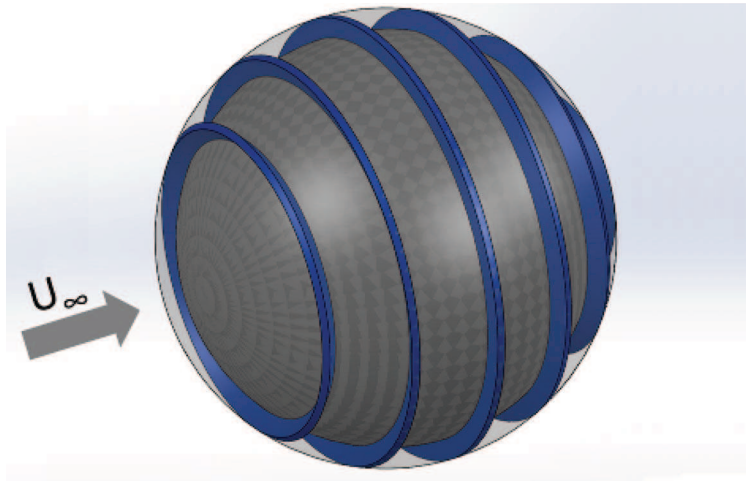
FIG. 11. Model of solid sphere with axisymmetric baffles and plastron.
