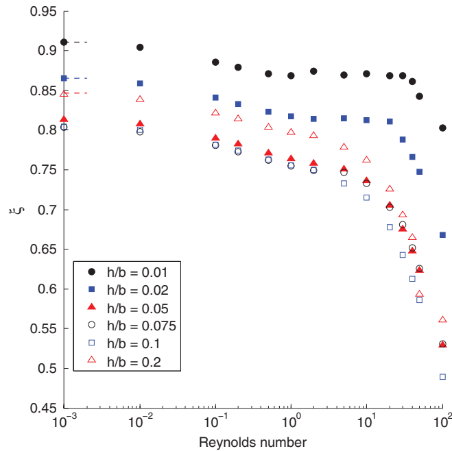
FIG. 8. Effect of the plastron on drag reduction factor ( \xi ) for a range of plastron thicknesses.
