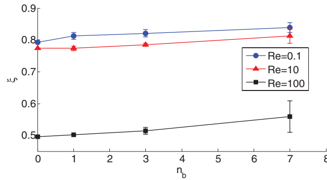
FIG. 15. Effect of addition of zero thickness baffles on drag reduction ( h/b = 0.1 ).
