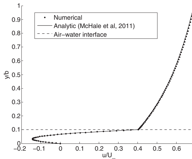
FIG. 7. Axial velocity at the top of the sphere ( Re = 0.001 , h/b = 0.1 ).
