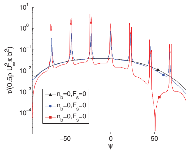
FIG. 19. Interfacial shear profiles for a range of baffle configurations ( Re = 100, h/b = 0.1 ).
