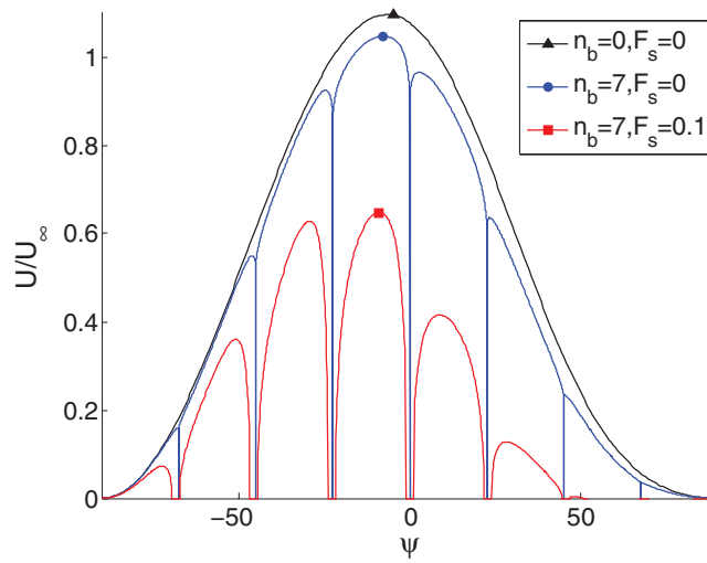
FIG. 18. Interfacial velocity profiles for a range of baffle configurations ( Re = 100, h/b = 0.1 ).
