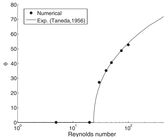
FIG. 5. Dependence of separation angle on Reynolds number for a solid sphere.
