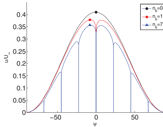
FIG. 13. Interfacial axial velocity component with zero thickness baffles ( Re = 0.1 , h/b = 0.1 ).
