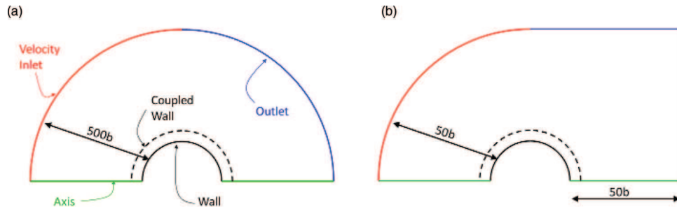
FIG. 2. Schematic of domain shape and size used for (a) low Reynolds number range and (b) high Reynolds number range (not to scale).
