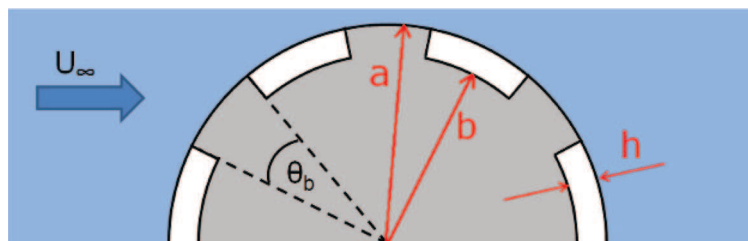
FIG. 10. Schematic of baffle configuration.
