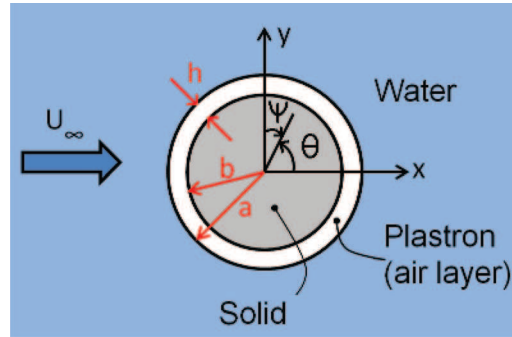
FIG. 1. Schematic of an encapsulated sphere.
