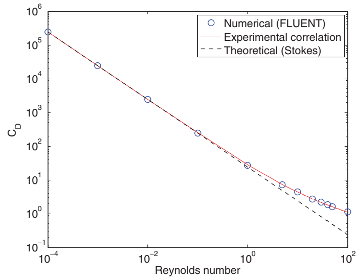
FIG. 4. Drag coefficient of solid sphere across a wide Reynolds number range.
