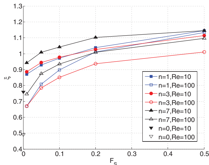
FIG. 16. Drag reduction for different baffle configurations at Re = 10 and Re = 100 ( h/b = 0.1 ).
