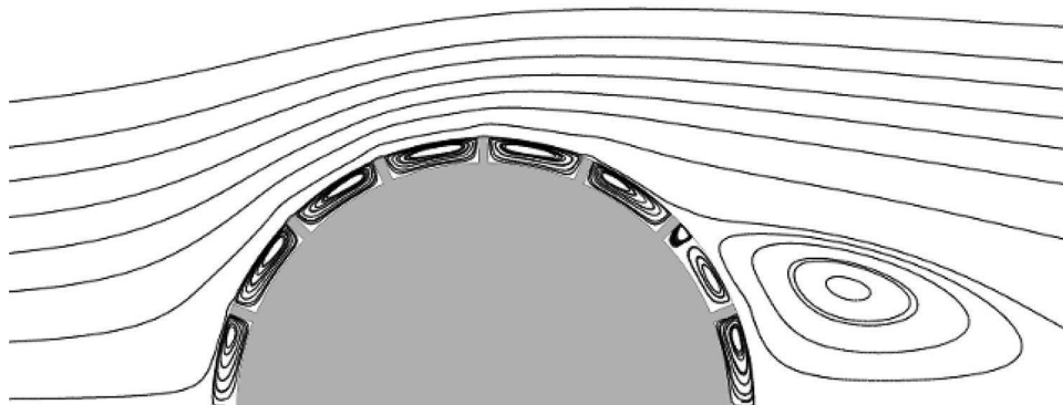
FIG. 20. Pathlines showing separation from the middle of a cavity section ( F_s = 0.1, Re = 100, h/b = 0.1 ).
