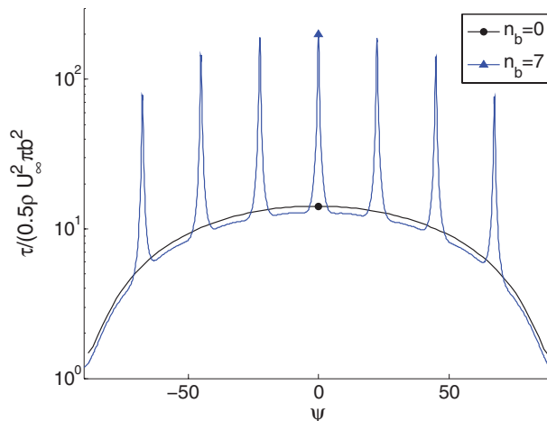
FIG. 14. Interfacial shear stress profiles with zero thickness baffles ( Re = 0.1 , h/b = 0.1 ).
