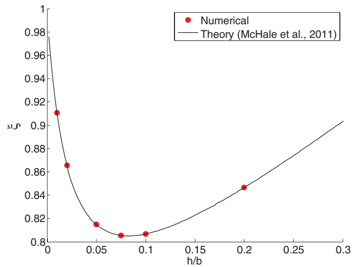
FIG. 6. Drag reduction due to plastron in Stokes flow.
