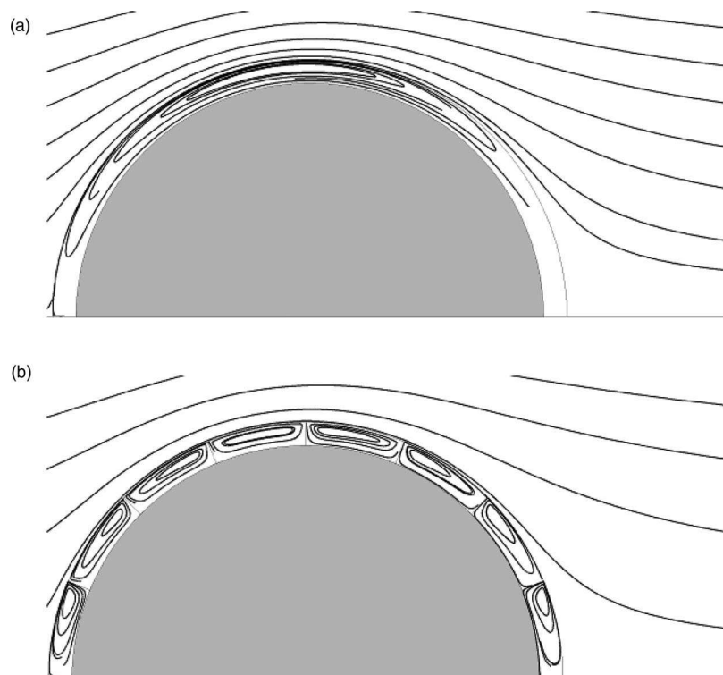
FIG. 12. Pathlines past an encapsulated sphere (a) without baffles and (b) with baffles ( Re = 100 ).
