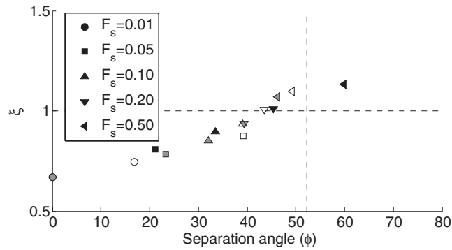
FIG. 17. Relation between separation angle and overall drag value ( Re = 100 , h/b = 0.1 ). White symbols: n_b = 1 , grey: n_b = 3 , black: n_b = 7 . The dashed line is for a no-slip sphere. 20
