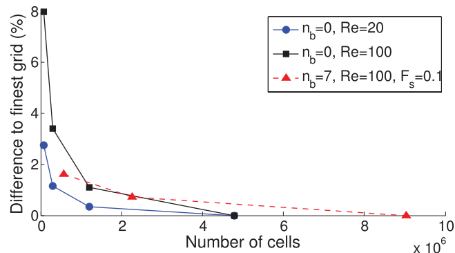
FIG. 3. Grid refinement study for a solid and plastron-encapsulated spheres.
