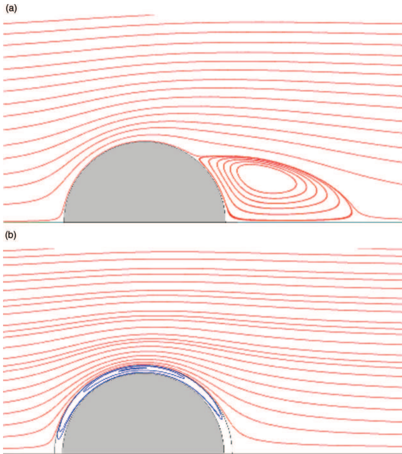
FIG. 9. Streamlines past (a) a solid sphere and (b) plastron-encapsulated sphere ( hb = 0.1 ) at Re = 100 showing separation suppression.
