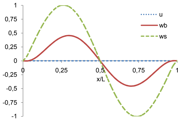
b. Second mode shape \omega_2 = 33.654 .
