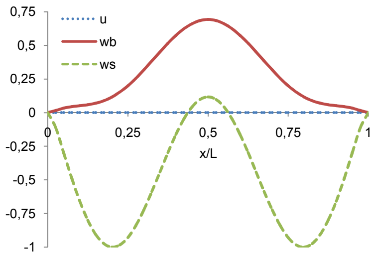
c. Third mode shape \omega_3 = 54.824 .
