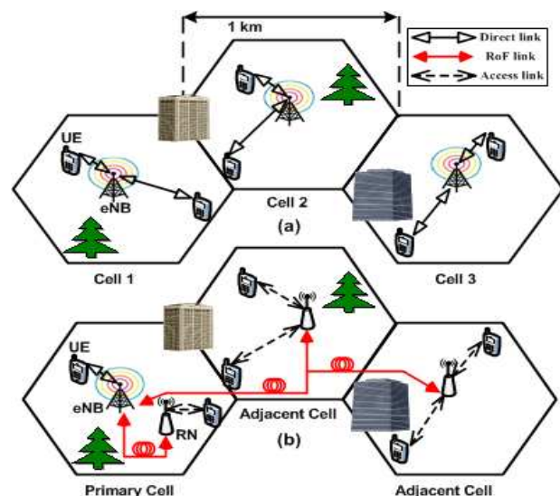
Fig. 1: LTE radio access network structure (a) without RN and (b) with RN in urban zone.
