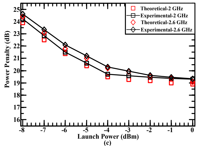
Fig. 5: OLP against power penalty analysis of (a) QPSK DD-FDM, (b) 16-QAM DD-FDM and (c) 64-QAM DD-FDM
