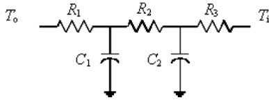
Figure 1: 2nd order lumped parameter construction element
