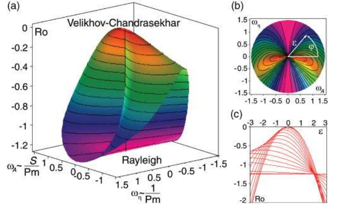
FIG. 1. (Color online) (a) The critical Rossby number of SMRI as a function of \omega_A \sim S \text{Pm}^{-1} and \omega_\eta \sim \text{Pm}^{-1} for \omega_v = 1 , \alpha = 1 , \Omega_0 = 1 , i.e., for \text{Re} = 1 . (b) Top view of the surface. (c) Cross sections of the surface along the rays specified by the Lundquist number, or, equivalently, by the angle \varphi that varies from 0 to 1.5 through the equal intervals \Delta\varphi = 0.1 ; the horizontal line corresponds to \varphi = \pi/2 . Note that negative values of \omega_\eta and \varepsilon are not physical.
