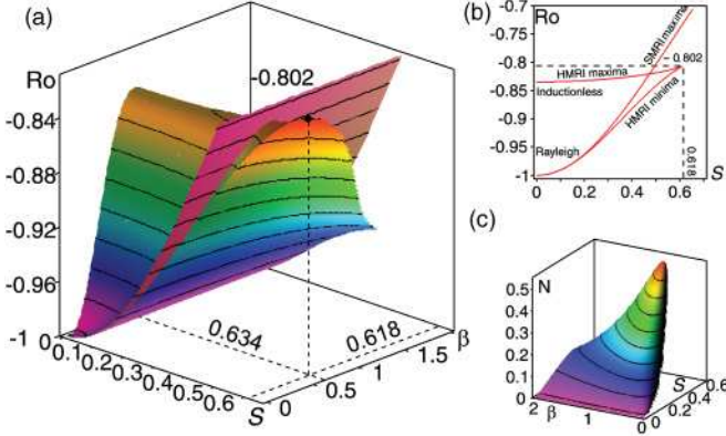
FIG. 3. (Color online) (a) Discriminant surface in the (S, \beta, Ro) space and (b) its cross section at \beta = 0.634 . (c) Interaction parameter N = S^2 Rm^{-1} at the essential HMRI maxima.
