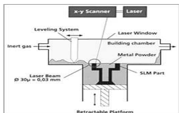
Fig. 5. The selective laser melting process 12
