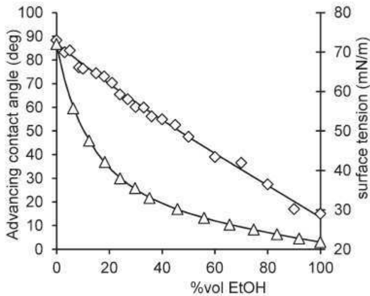
Figure 2. Advancing contact angle (measured on CTMS modified glass slides) and surface tensions of ethanol solutions in water used for MED tests (Literature values shown are taken from reference 12).
