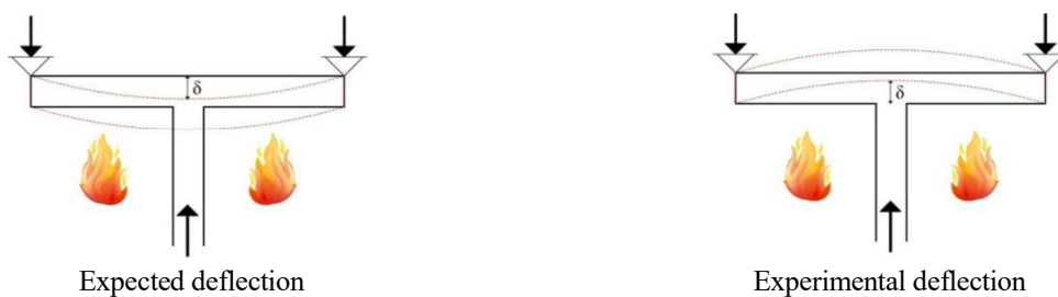
Figure 2 Conceptual arrangement for testing heated flat plate beam-column connections.
