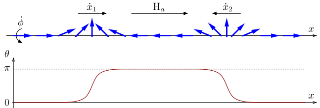
FIG. 1: (Color online) Dynamics of domain walls. See text for discussion.
