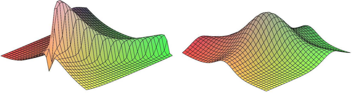
Figure 1: Graph of the height function h(t, x, y) for the rank-2 solution of the SS type (3.69) at times t = -\pi/5 and t = 0 .
