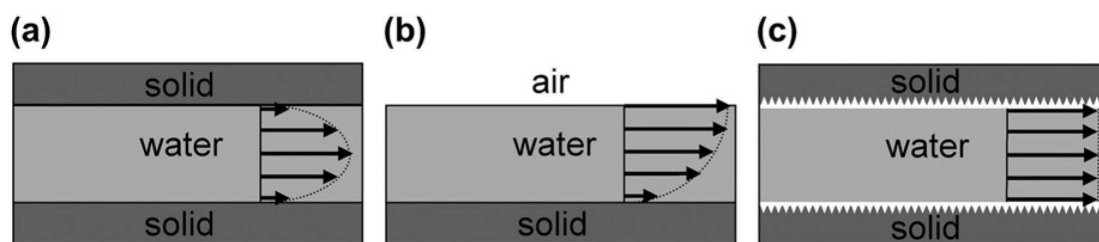
Fig. 2 – Schematics of the cross-section of laminar flow through: (a) a tube with no-slip boundary conditions and high frictional drag at the walls, (b) a half-tube with a lower frictional drag at the air-water interface, and (c) a tube with a superhydrophobic interface providing a boundary with composite water-solid and water-air interfaces dominated by low frictional drag at the water-air interfaces.
