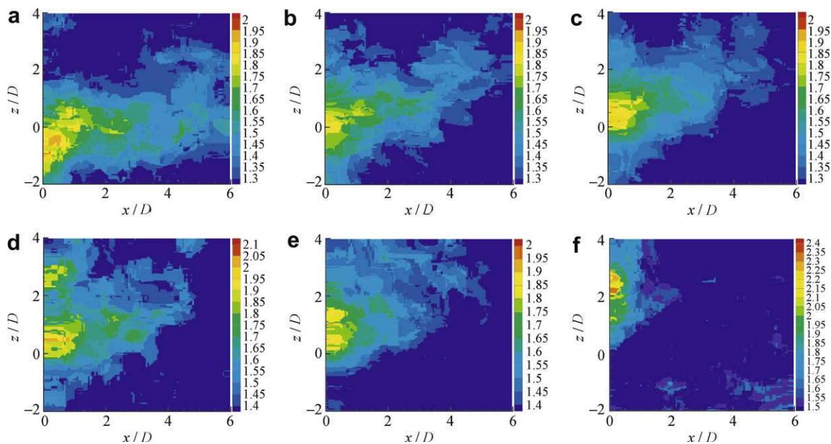
Fig. 9. Heat transfer coefficient h_g/h_0 for air injection at Re_D = 3191 and M = 1.2 . (a) Rt = 0.0094 , PS; (b) Rt = 0.0155 , PS; (c) Rt = 0.0249 , PS; (d) Rt = 0.0094 , SS; (e) Rt = 0.0155 , SS; and (f) Rt = 0.0249 , SS.
