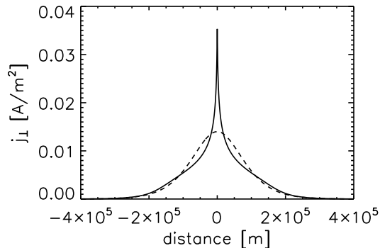
Fig. 1.— Perpendicular current density profiles at 43 seconds (solid line) and t = 0 (broken line) obtained with \eta_{\perp} = 61.86 \Omega\text{m} for the Harris current sheet.
