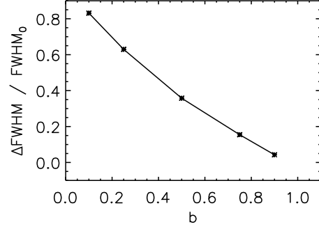
Fig. 8.— The change in the FWHM measurement as a function of b in Equation (10). \Delta\text{FWHM} = |\text{FWHM}_{400} - \text{FWHM}_0| , measured at 400 seconds and initialisation.
