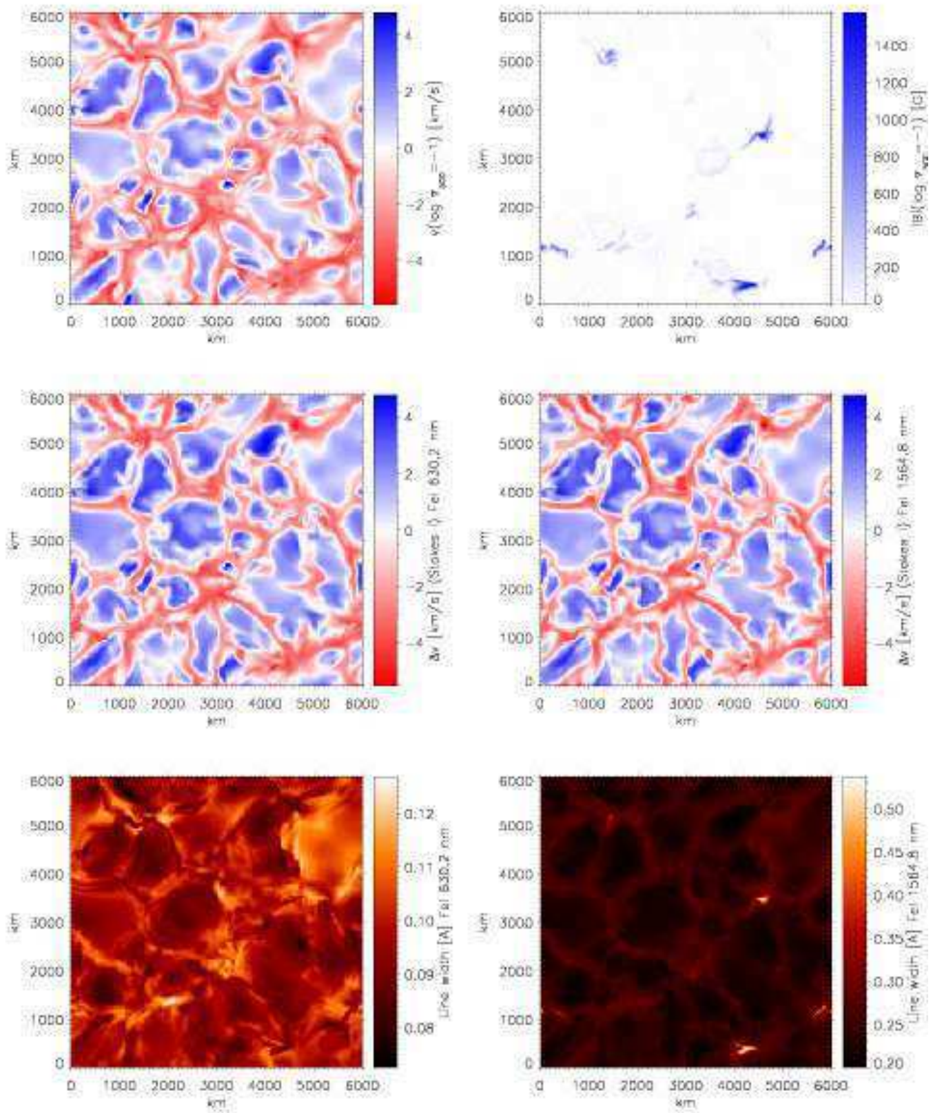
Fig. 8. Same as Fig. 7 for the \langle B_z \rangle = 10\text{ G} simulation.
