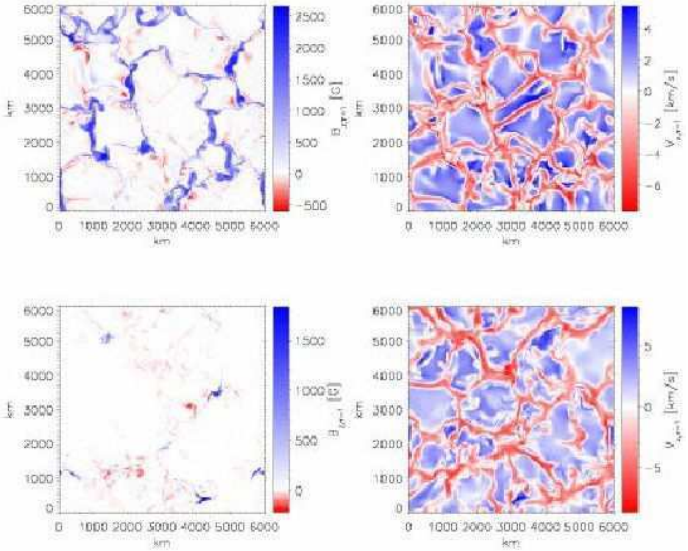
Fig. 1. Vertical magnetic field component (left panels) and vertical velocity (right panels) on the surface \tau_{500} = 1 (continuum optical depth unity at 500 nm wavelength) for snapshots from simulations with \langle B_z \rangle = 200\text{ G} (plage, upper row) and \langle B_z \rangle = 10\text{ G} (decay phase, bottom row). Positive values of the velocity (shown in blue) correspond to upflows; downflows are indicated in red. Note the different scales for positive and negative B_z in the left panel (all negative-polarity field is rather weak).
