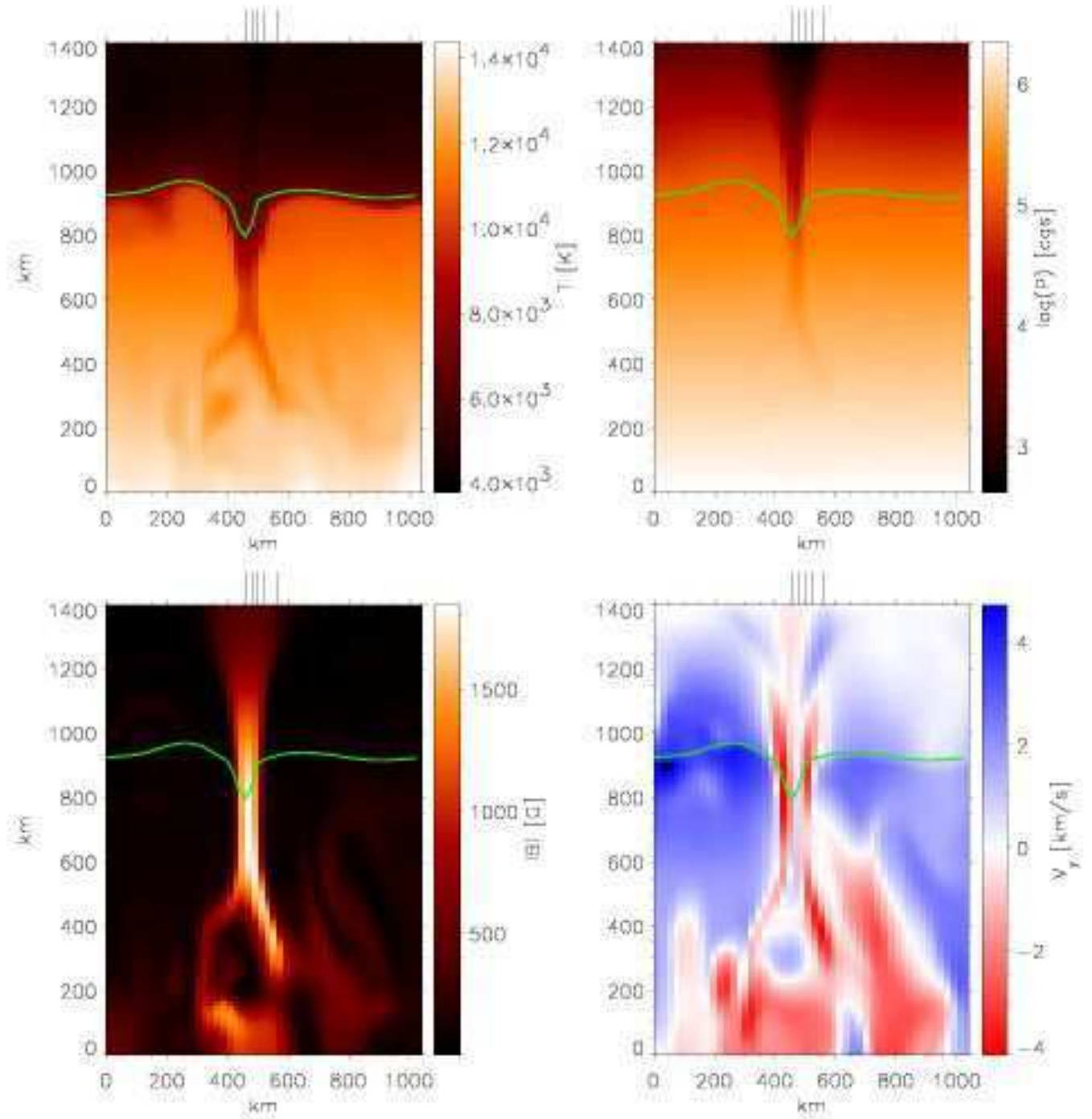
Fig. 10. Temperature (upper left panel), gas pressure (upper right panel), magnetic field strength (lower left panel), and vertical velocity (lower right panel) for the vertical cut through the simulation box marked by the white line on the upper left panel of Fig. 3. The green curve indicates the level \tau_{500} = 1 . Negative values of the velocity (shown in red) correspond to downflows. The lines of sight corresponding to the Stokes profiles and gradients shown in Fig. 11 are indicated at the top of each panel.
