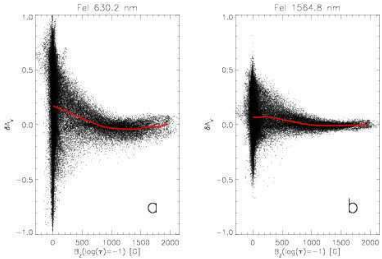
Fig. 15. Scatter plots of the Stokes- V area asymmetry versus the vertical (line-of-sight) component of the magnetic field at \tau_{500} = 0.1 a : FeI 630.2 nm, b : FeI 1564.8 nm. The lines show binned averages.
