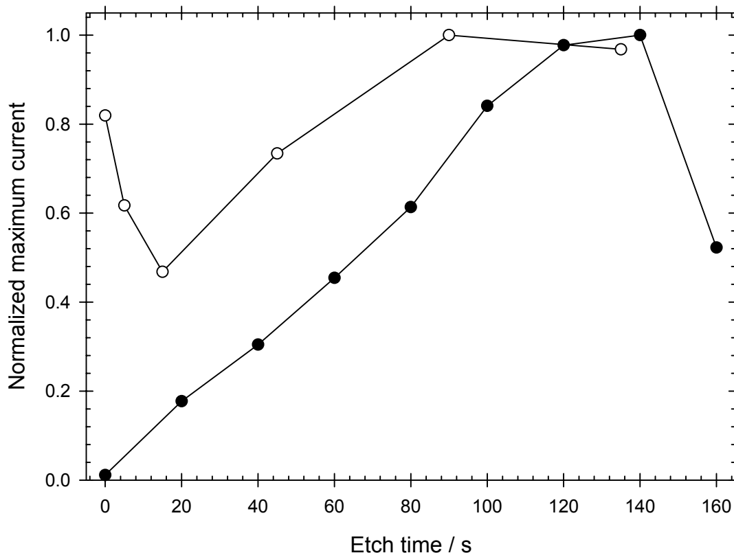
Figure 3. Graph showing normalized photocurrent response to pulsed green LED illumination for ED-CuInSe 2 (○) and SP-CuInSe 2 (●) films. All photocurrents were measured at -0.3 vs Ag|AgCl / V in aqueous 0.2 M \text{Eu}^{3+} electrolyte at pH 2.
