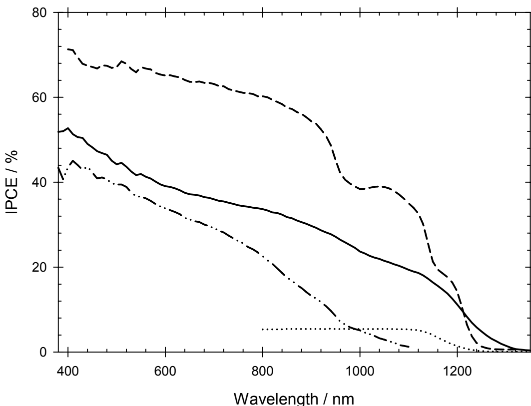
Figure 8. IPCE spectra of ED-CuInSe 2 (—), ED-Cu(In,Ga)Se 2 (····), SP-CuInSe 2 (---), and CuInS 2 (-·-·-). Applied potentials and chopping frequencies were optimised to give the maximum photo-response. All films were measured in 0.2 M Eu 3+ solution.
