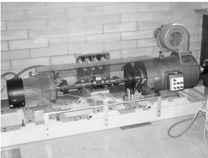
Fig. 16. The dynamometer to be used for the testing
