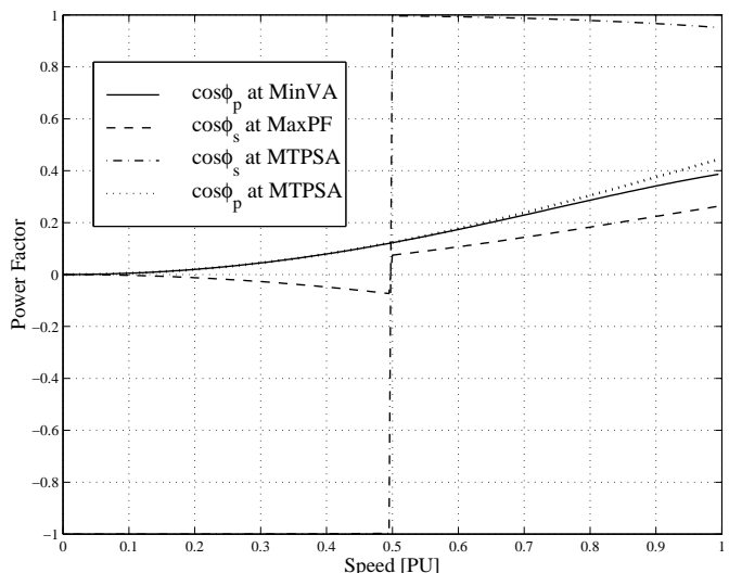
Fig. 11. Power factor performance for control strategies investigated
