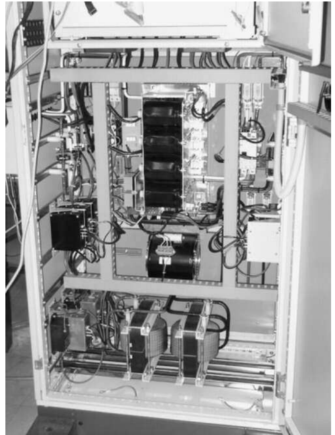
Fig. 14. The power electronics for the experimental system
