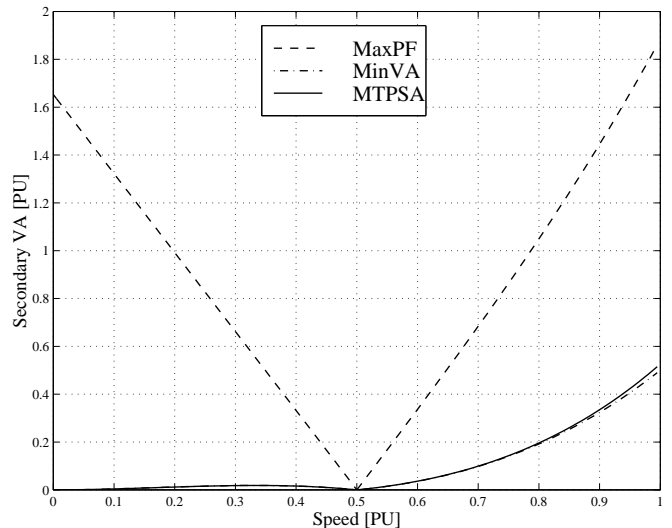
Fig. 10. Inverter VA requirements for various control strategies
