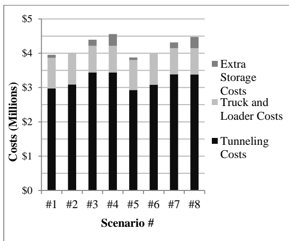
Figure 7: Cost results of the examined scenarios
