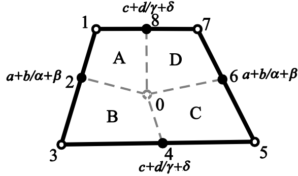
Fig. 11 A special configuration of Bennett linkage from the reconfigurable Bennett network.
