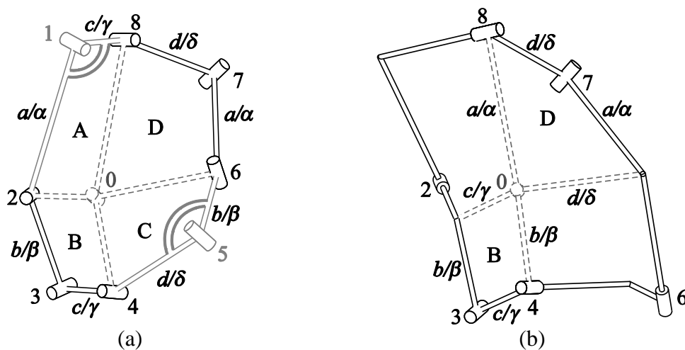
Fig. 6 The modification of the Bennett network into Case IV linkage: (a) the schematics of the modification process of Case IV linkage; (b) linkage identification for the Case IV linkage.
