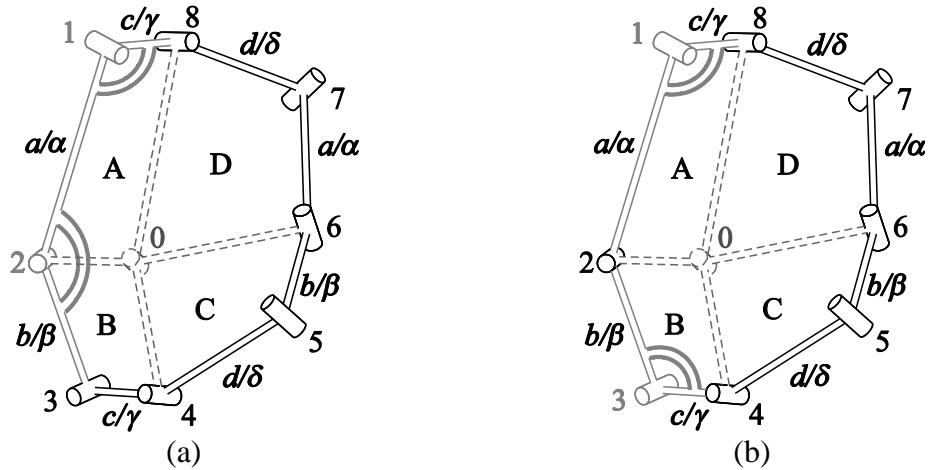
Fig. 4 The modification of the Bennett network into Cases I & II linkages: (a) the Case I linkage with joints 1 and 2 fixed and (b) the Case II linkage with joints 1 and 3 fixed.
