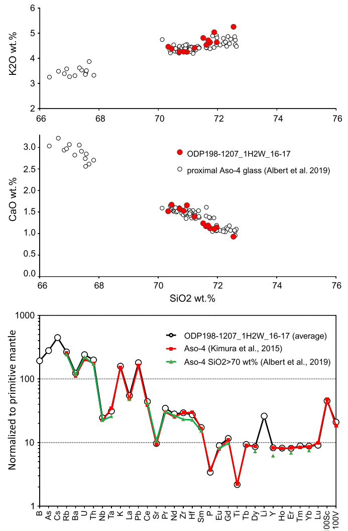
Fig. 2. Composition of glass from tephra sample ODP198 core 1207A, section 1H2W, interval of 16-17 cm (166-167 cm below sea floor) and proximal Aso-4 samples (Kimura et al., 2015; Albert et al., 2019). Albert et al. (2019) analyzed pumice from three levels: base, middle and upper. Low-Si glass occurs only in the upper level; fallout from this later phase of the Aso-4 eruption did not pass over ODP1207.
