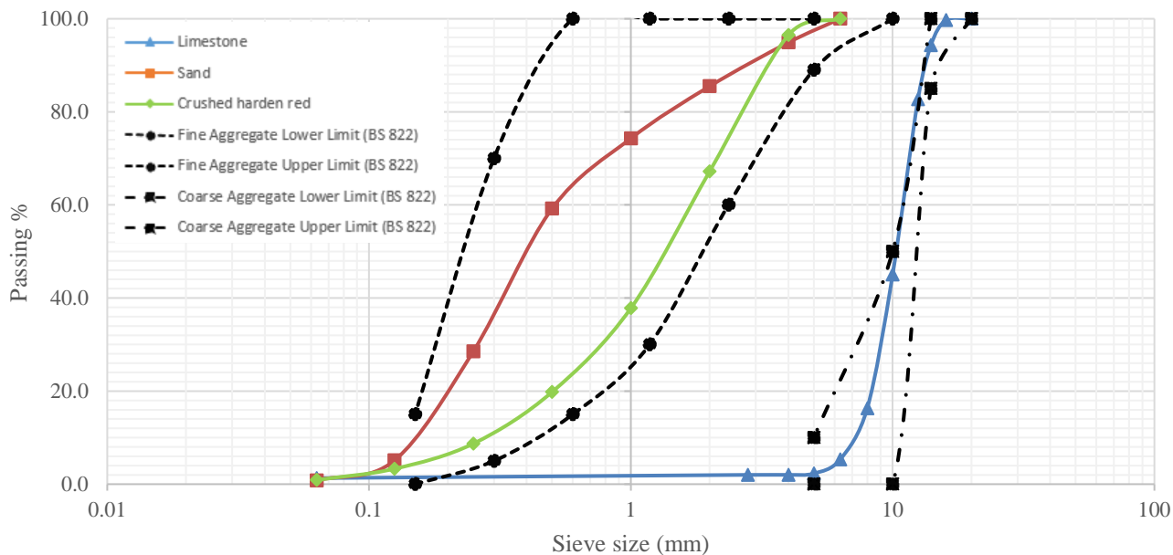
Fig. 2: Sieve analysis of fine and coarse aggregate.
