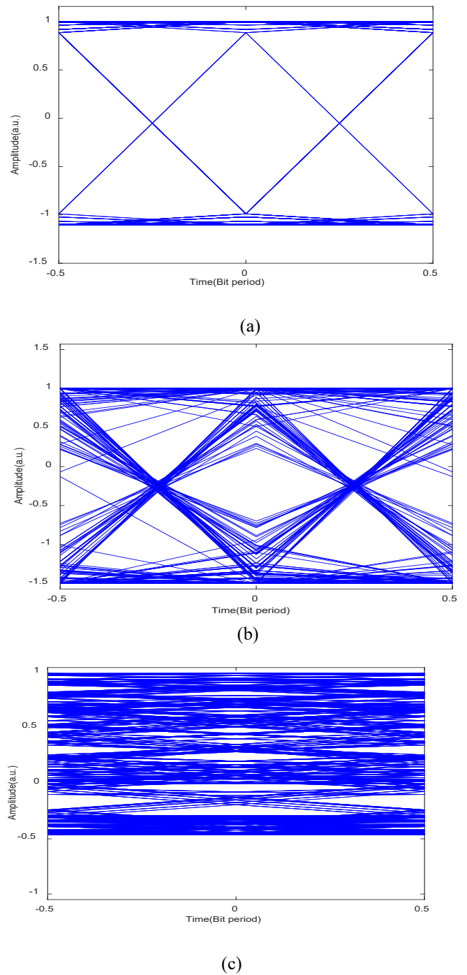
Fig.9. Eye diagrams of the received optical signal at different link-spans: (a) 2m, (b) 6m and (c) 12m.
