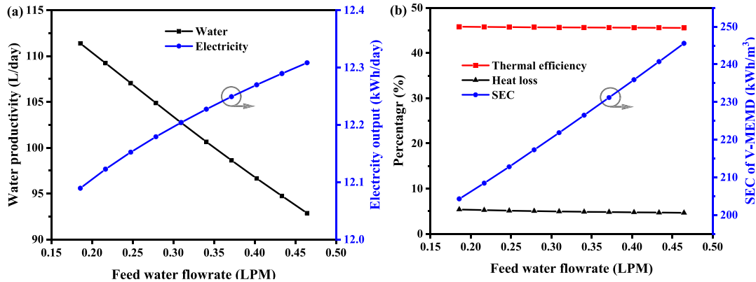
Fig. 11. Effect of feed water flowrate on (a) water productivity and electricity generation, and (b) thermal efficiency, heat loss and desalination SEC. Hot water flowrate is 9.6 LPM, and the tank diameter is 0.5 m
