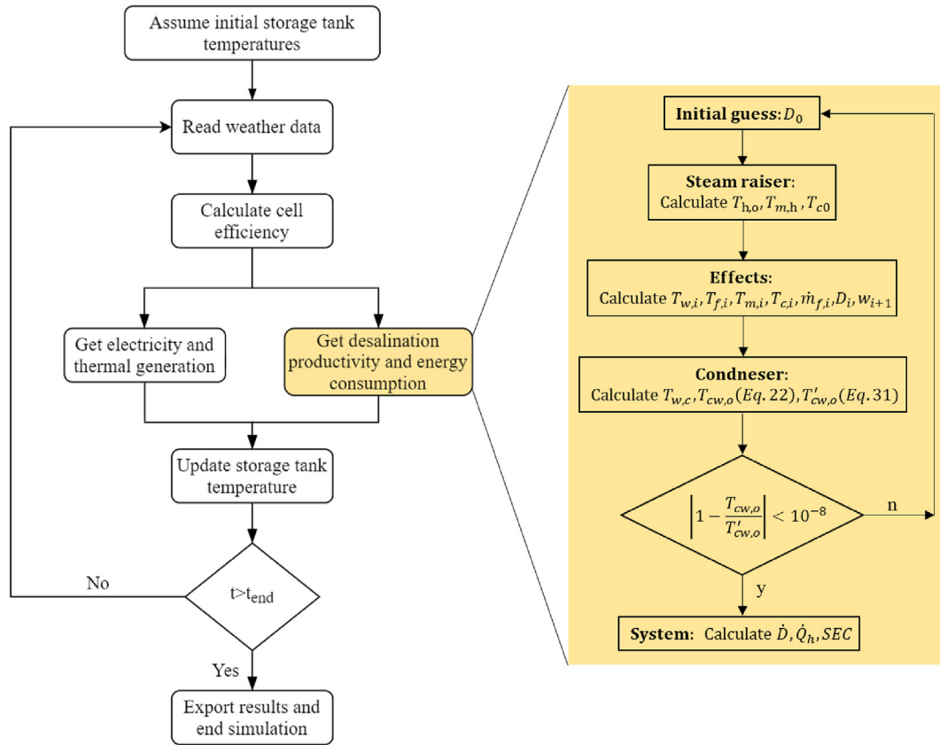
Fig. 6. Schematic of the solution algorithm.
