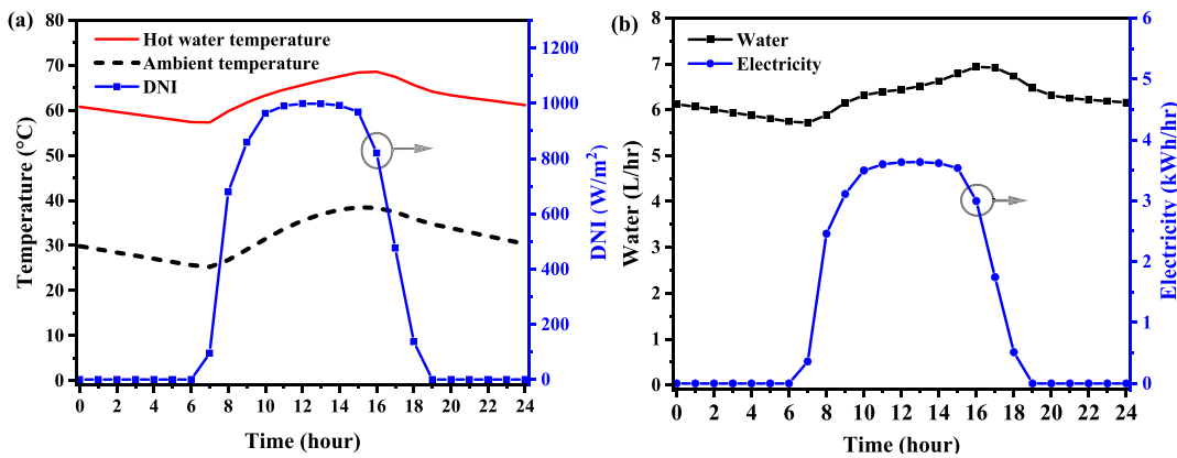
Fig. 7. Daily profile of (a) solar radiation and water temperatures, and (b) water production rate and electricity generation on a typical day (Oct-15).
