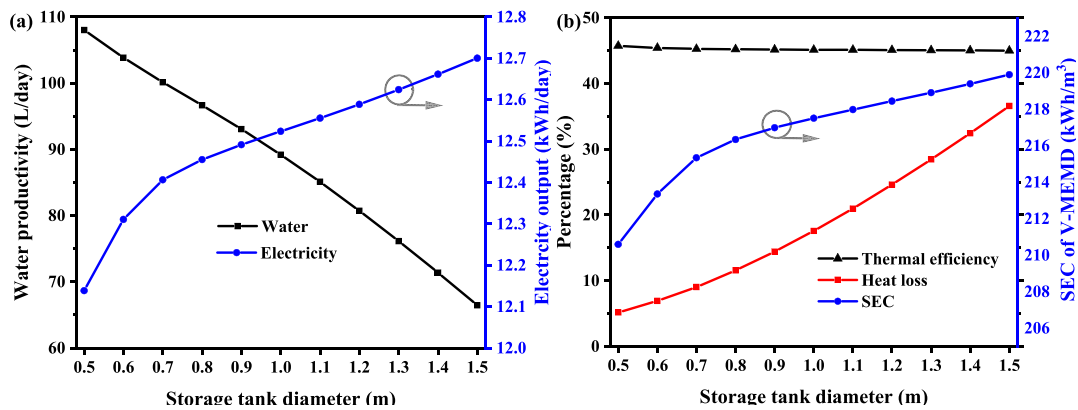
Fig. 12. Effect of storage tank diameter on (a) water productivity and electricity generation, and (b) thermal efficiency, heat loss and desalination SEC. Hot water flowrate is 9.6 LPM, and feed flowrate is 0.3 LPM.
