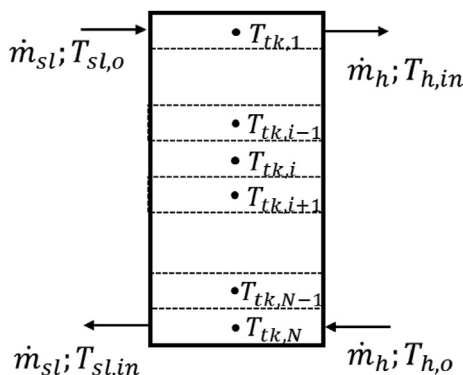
Fig. 5. Model schematic for the heat storage tank.
