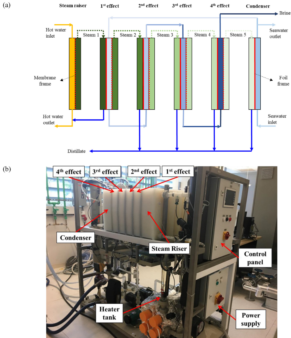
Fig. 3. (a) Schematic diagram of the vacuum multi-effect membrane distillation system; (b) pictorial view of a four-effect V-MEMD module.
