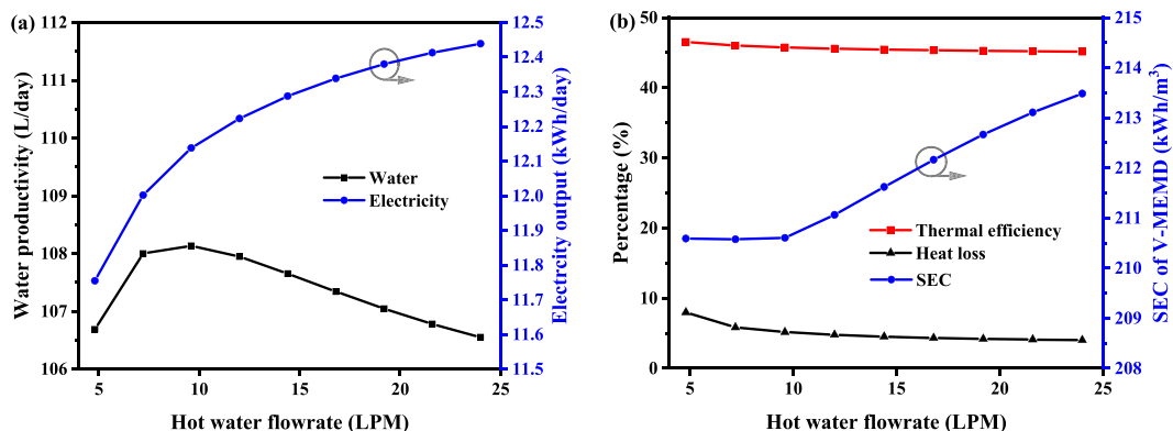
Fig. 10. Effect of hot water flowrate on (a) water productivity and electricity generation, and (b) thermal efficiency, heat loss and desalination SEC. The storage tank diameter is 0.5 m, and the feed water flowrate is 1/30 of the hot water flowrate.
