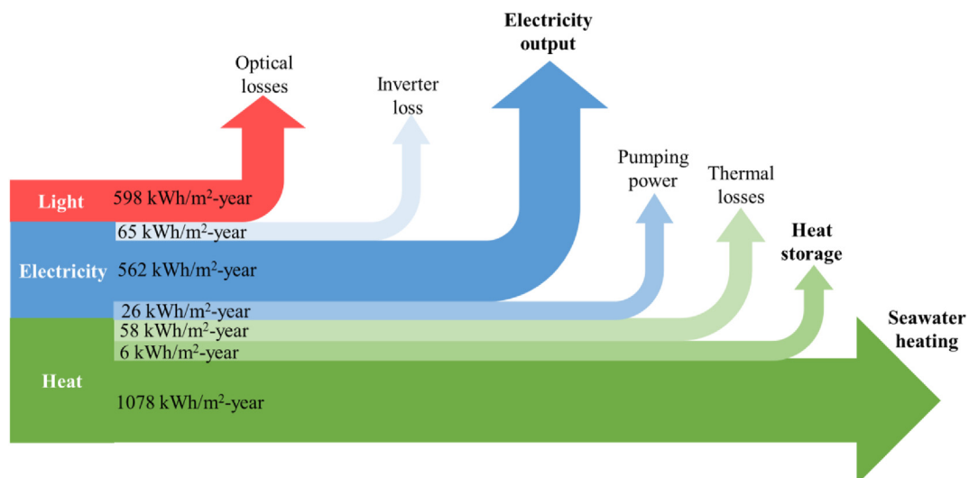
Fig. 8. Energy collection, utilization, and losses diagram for the proposed system on an annual basis.
