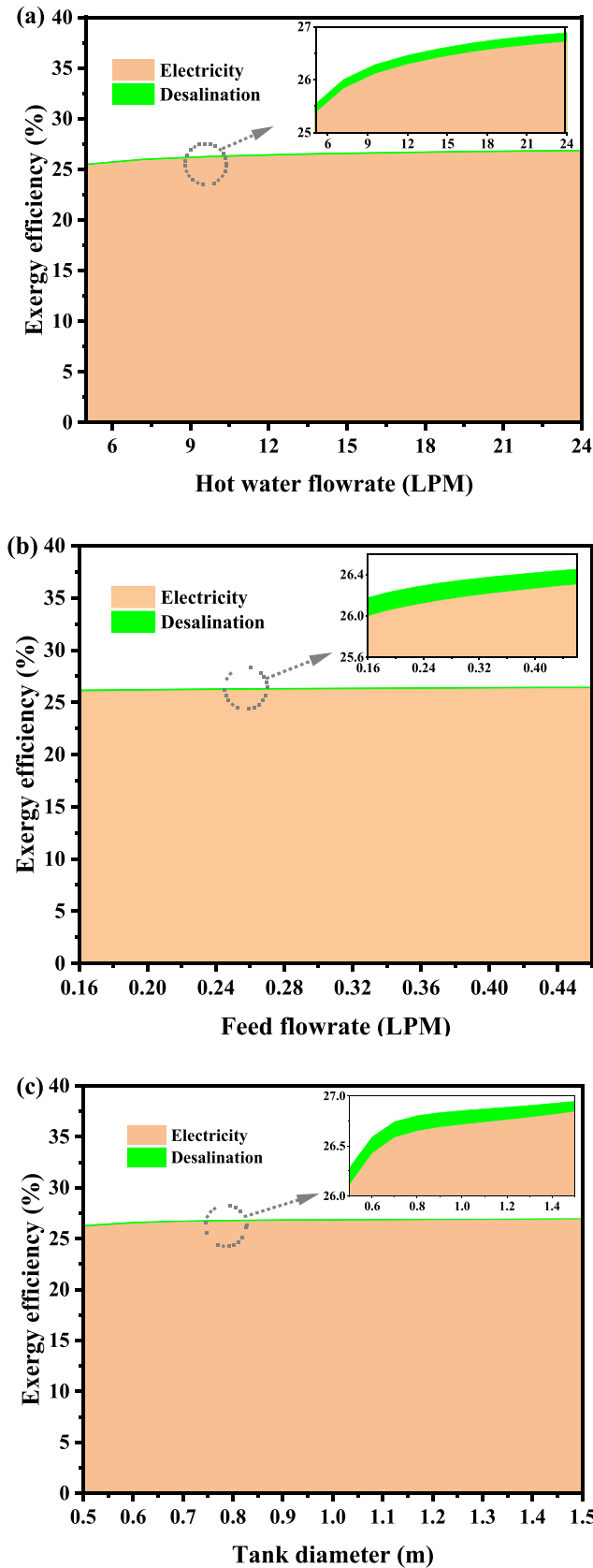
Fig. 13. Exergy efficiency of the system under different (a) hot water flowrate, (b) feed flowrate and (c) tank diameter.
