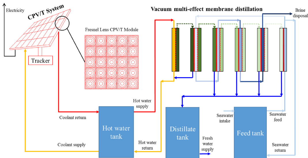
Fig. 1. Schematic diagram of the proposed solar-driven electricity/water cogeneration system.
