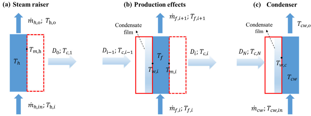
Fig. 4. Model schematic for the V-MEMD module, (a) steam raiser, (b) production stages, and (c) condenser.
