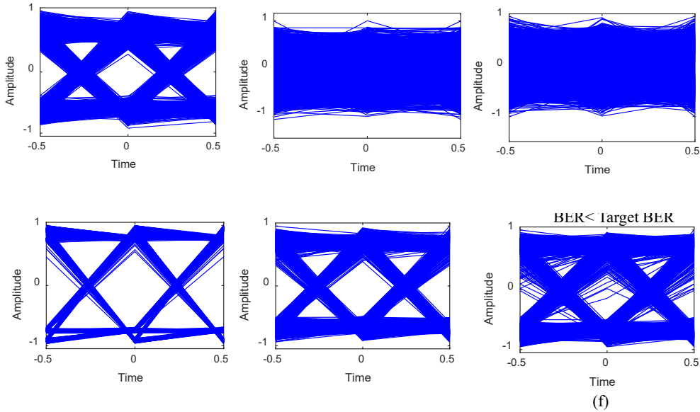
Fig. 2: Measured eye diagrams for R_b of 250 kb/s for: (a) AF and (b) DF with L_s of 12 m, and (c) AF and (d) DF with L_s of 16 m; and R_b of 500 kb/s for: (e) AF and (f) DF with L_s of 16 m
