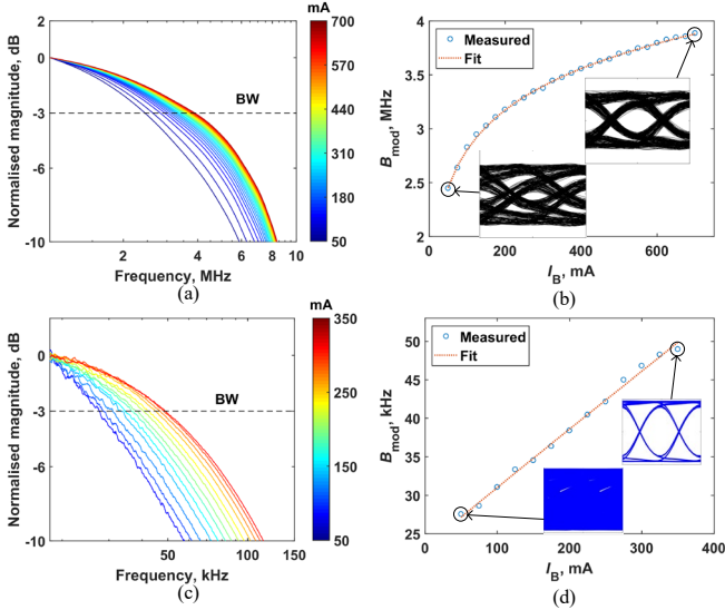
Fig. 6 DUT transient analysis, measured frequency response with stepped I_B for (a) WPLED and (c) OLED1; and extracted B_{mod} vs. I_B for (b) WPLED (inset eyediagrams at 10 Mb/s for min and max I_B ) and (d) OLED1 (inset eyediagrams at 100 kb/s for min and max I_B ).
