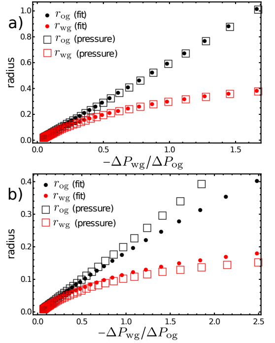
FIG. 3. The lubricant-drop and lubricant-gas curvature radii as function of the pressure ratio -\Delta P_{\text{wg}}/\Delta P_{\text{og}} for the 2D (panel a) and 3D (panel b) cases. Two measures for the curvature radii are presented, by inverting the Laplace pressures measured and through fitting the interface shapes with circular arcs. The parameters used here are \theta_{\text{o}} = 40^\circ , \theta_{\text{w}} = 160^\circ , \theta_{\text{g}} = 160^\circ , \theta_{\text{ow}}^{\text{CB}} = 15^\circ and \theta_{\text{og}}^{\text{CB}} = 15^\circ .
