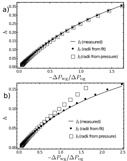
FIG. 4. Comparison of the measured lubricant ridge h with those computed according to Eq. (5). The radii r_{ow} and r_{og} can be obtained by fitting the interfaces with circular arcs or by inverting the Laplace pressures, as shown in Fig. 3. The parameters used here are \theta_o = 40^\circ , \theta_w = 160^\circ , \theta_g = 160^\circ , \theta_{ow}^{CB} = 15^\circ and \theta_{og}^{CB} = 15^\circ . Panel a) 2D; panel b) 3D.
