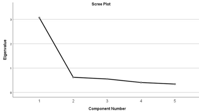
Figure 3. Factor Analysis Scree Plot.
