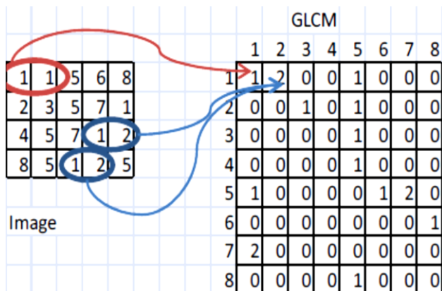
Fig. 2. GLCM calculation from 4-by-5 image I [23].
