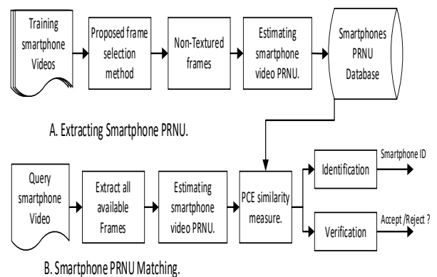
Fig. 1. High-level of the proposed source smartphone video identification and verification system.
