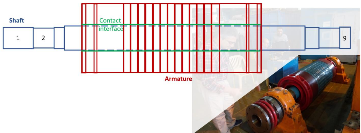
Figure 2- the rotor-armature structure
