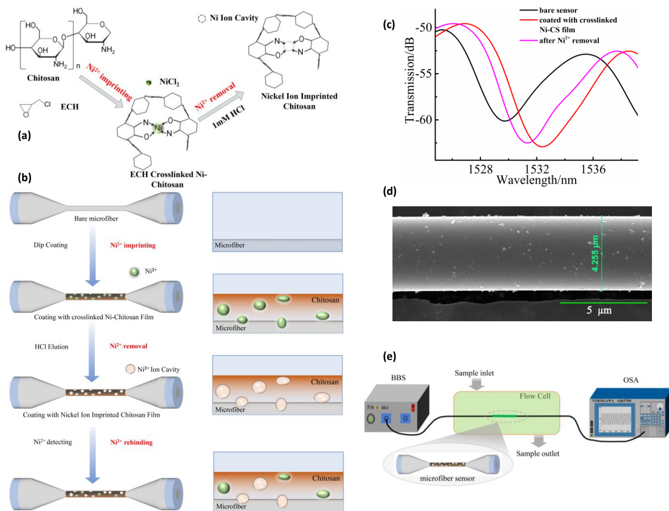
Fig. 2 (a) \text{Ni}^{2+} -II-CS synthesis scheme. (b) Procedure for obtaining the microfiber sensor coated with \text{Ni}^{2+} -II-CS film. (c) STNCS sensor response curves for a bare sensor, a sensor coated with Ni-CS film, and a sensor coated with \text{Ni}^{2+} -II-CS film (after \text{Ni}^{2+} removal). (d) SEM image of the STNCS sensor. (e) Schematic diagram of the sensing system.
