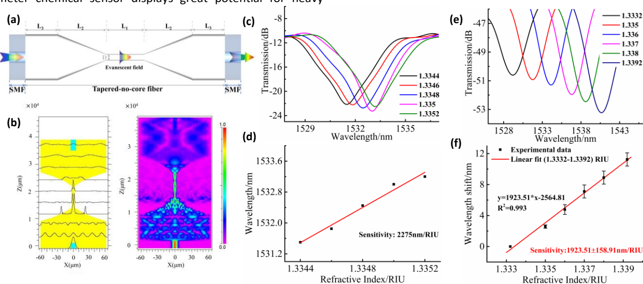
Fig. 1 (a) Schematic diagram of the STNCS sensor. (b) Optical field distribution and normalized optical intensity propagating along the STNCS structure with a tapered waist diameter of 4.8 \mu\text{m} . (c) Simulated spectral response. (d) Simulated RI sensitivity predicted for the STNCS structure with 4.8 \mu\text{m} taper waist diameter in the RI range of about 1.334. (e) The STNCS sensor spectral response curves with different external RI values. (f) Sensitivity of the STNCS sensor to external RI (Error bars represent standard deviations for three repeated experiments).
