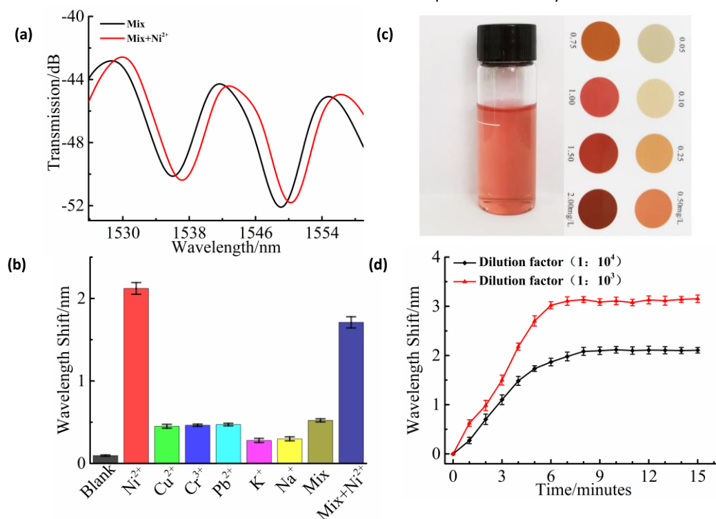
Fig. 4 (a) Spectral response of the STNCS sensor coated with \text{Ni}^{2+} -II-CS to the mix and the mix excess added \text{Ni}^{2+} sample. (b) Shift in dip wavelength of the STNCS sensor coated with \text{Ni}^{2+} -II-CS caused by exposure to various targets in lake water sample: blank, the 100nM excess of other cations including \text{Ni}^{2+} , \text{Cu}^{2+} , \text{Cr}^{3+} , \text{Pb}^{2+} , \text{K}^+ , \text{Na}^+ , mix and mix added \text{Ni}^{2+} . (c) Calibration of the \text{Ni}^{2+} content in electroplating wastewater sample by colorimetric test paper and (d) Shift in dip wavelength of the STNCS sensor coated with \text{Ni}^{2+} -II-CS caused by exposure to different concentrations of \text{Ni}^{2+} in electroplating wastewater sample. (Error bars represent standard deviations for three parallel experiments)
