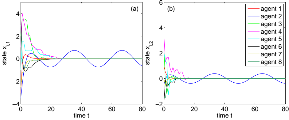
Figure 2. Resilient tracking consensus over the 2-dimensional state space with the leader agent 1 (red) and the Byzantine agent 2 (blue).
